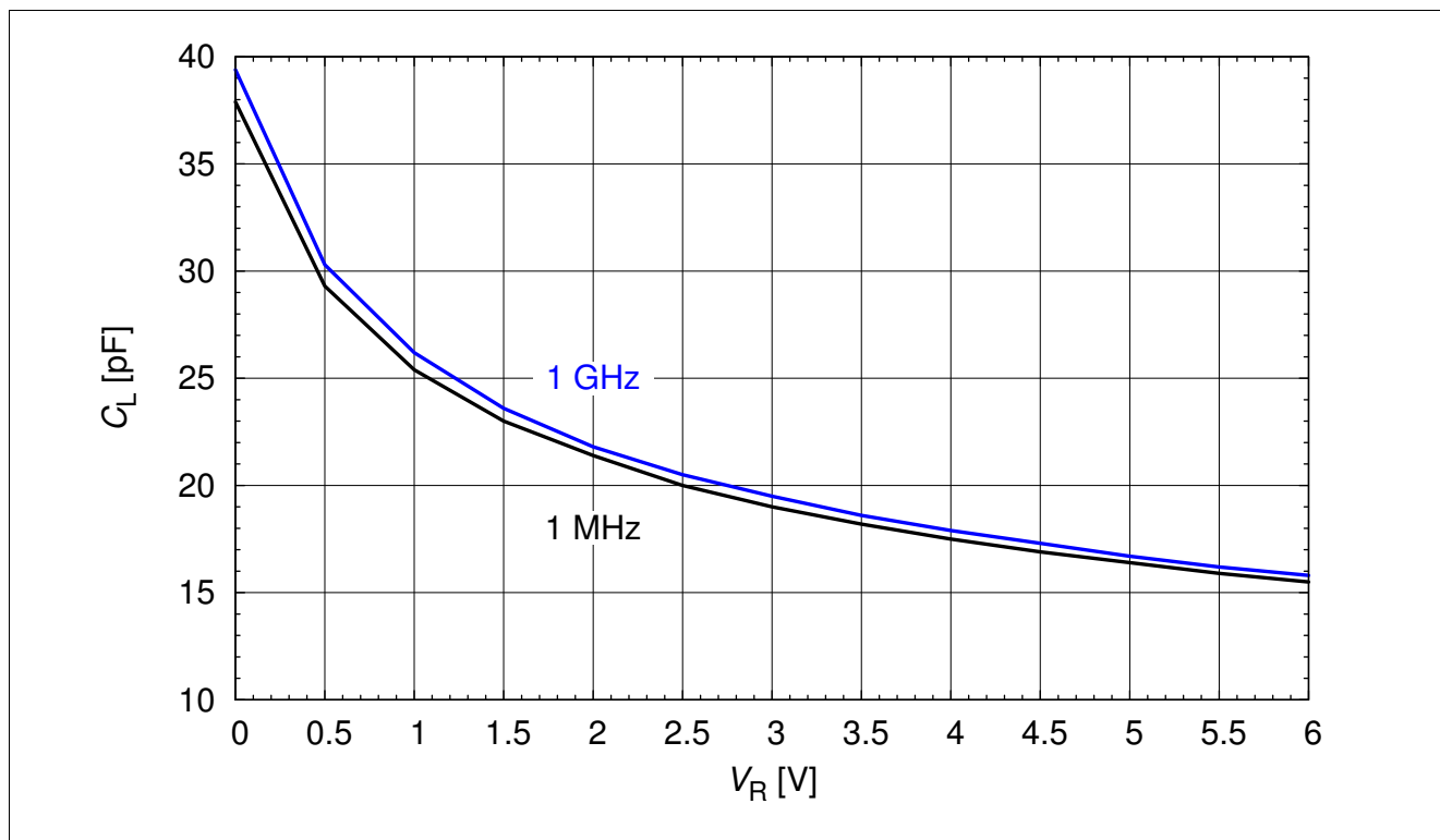
Figure 4-4 Line capacitance: C_L = f(V_R)
