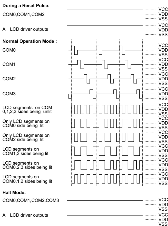
LCD driver output (1/4 duty, 1/2 bias)
