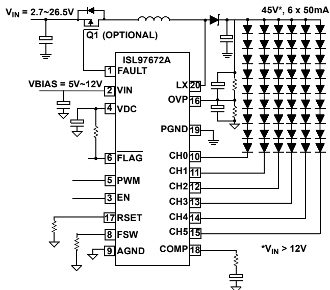
FIGURE 23. DUAL SUPPLY 2.7V OPERATION
