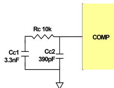
FIGURE 24. COMPENSATION CIRCUIT
