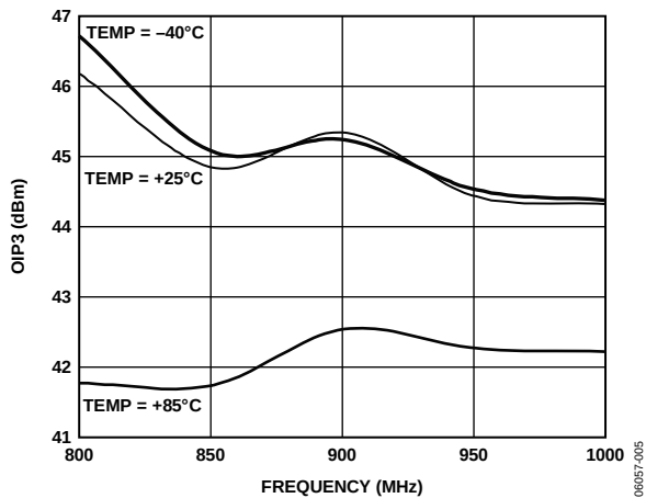
Figure 5. OIP3 vs. Frequency, V_{CC} = 5V , T_A = -40^\circ C, +25^\circ C, \text{ and } +85^\circ C
