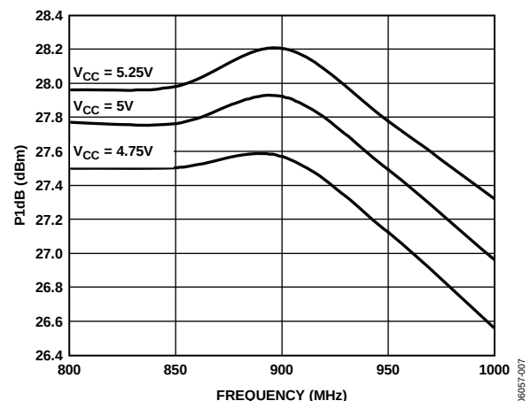
Figure 7. P1 dB vs. Frequency, V_{CC} = 4.75V, 5V, \text{ and } 5.25V , T_A = 25^\circ C
