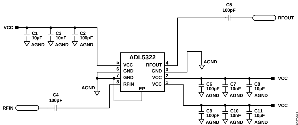
Figure 14. Basic Connections
