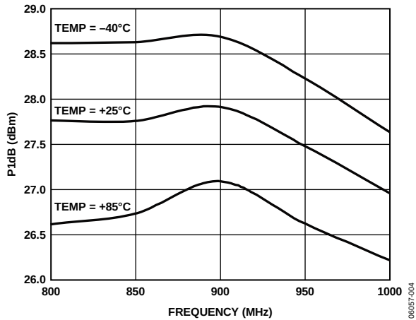
Figure 4. P1 dB vs. Frequency, V_{CC} = 5V , T_A = -40^\circ C, +25^\circ C, \text{ and } +85^\circ C
