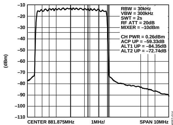
Figure 13. Spectrum of 4 Adjacent CDMA2000 Carriers Centered at 880 MHz; Total Carrier Power = 6 dBm (0 dBm per Carrier)
