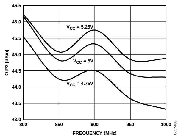
Figure 8. OIP3 vs. Frequency, V_{CC} = 4.75V, 5V, \text{ and } 5.25V , T_A = 25^\circ C
