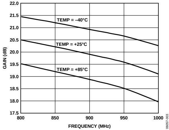
Figure 3. Gain vs. Frequency, V_{CC} = 5V , T_A = -40^\circ C, +25^\circ C, \text{ and } +85^\circ C
