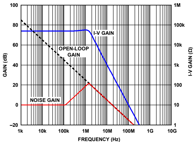
Figure 82. Compensating the TIA, C_F = 2.2 pF
