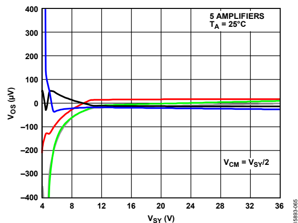
Figure 66. V_{OS} vs. V_{SY}
