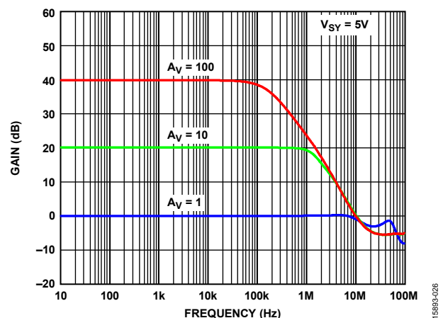
Figure 27. Gain vs. Frequency for Various Closed-Loop Gains, V_{SY} = 5 V
