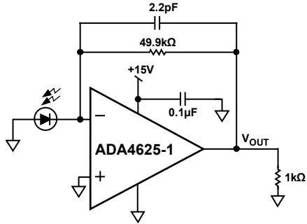
Figure 81. Single-Supply TIA Circuit Using the ADA4625-1
