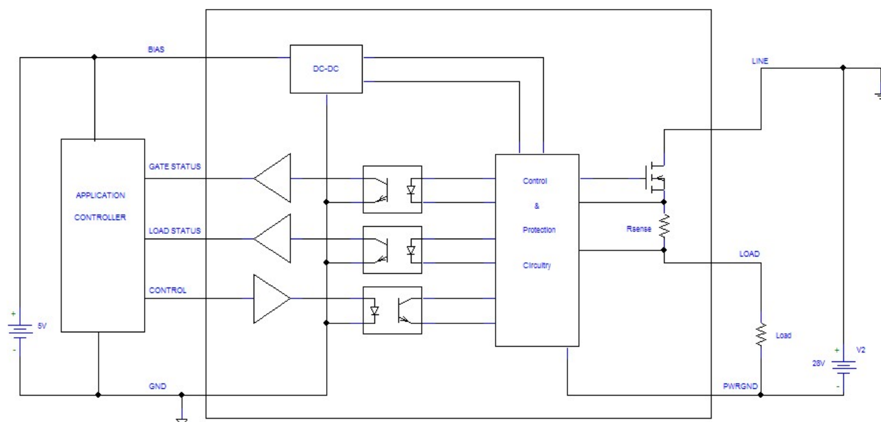
Figure 8 – Low Side Switch, Negative Supply
