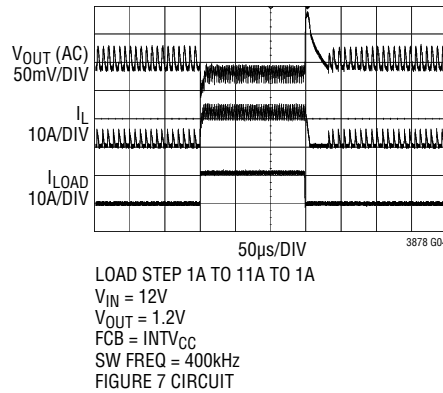
Transient Response DCM (Discontinuous Mode)
