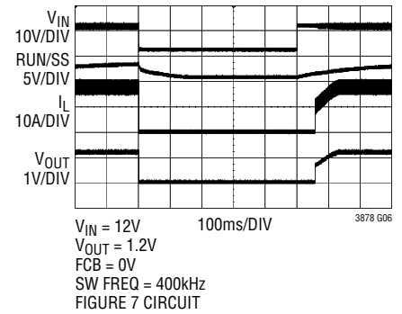
Start-Up V_{IN} Cycled Low and High
