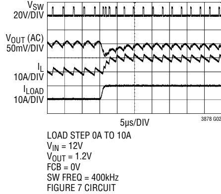
Transient Response FCM Positive Load Step
