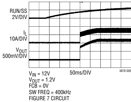
Normal Start-Up, RUN/SS Release from Zero
