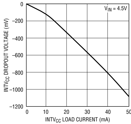
INTV_{CC} Dropout
