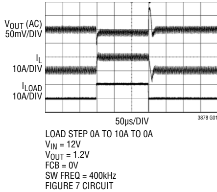
Transient Response FCM (Forced Continuous Mode)
