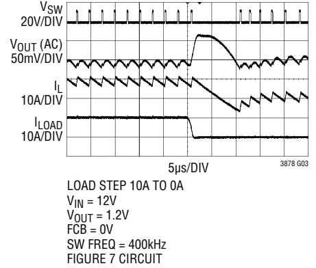
Transient Response FCM Negative Load Step
