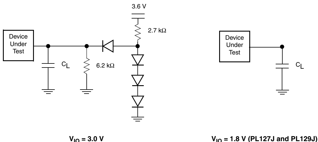
Figure 20.1 Test Setups
