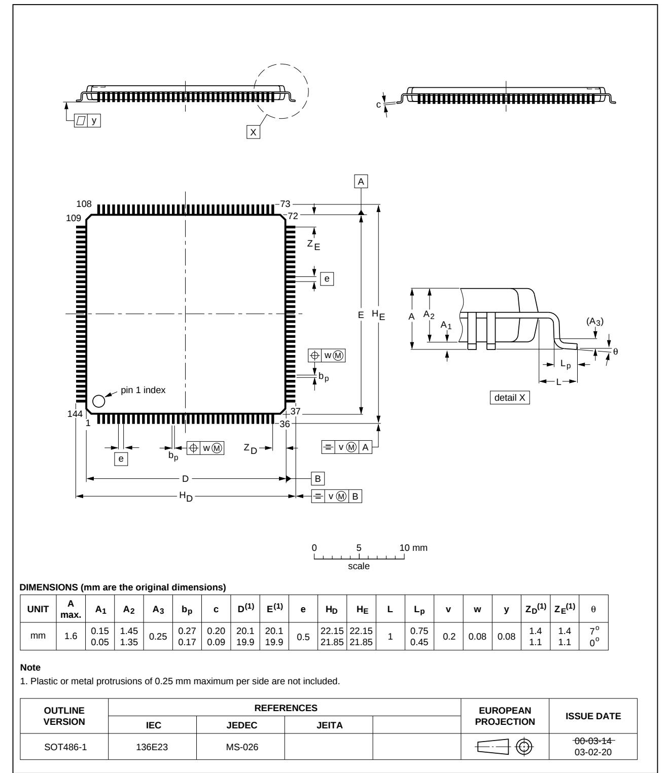
Fig 48. Package outline SOT486-1 (LQFP144)
