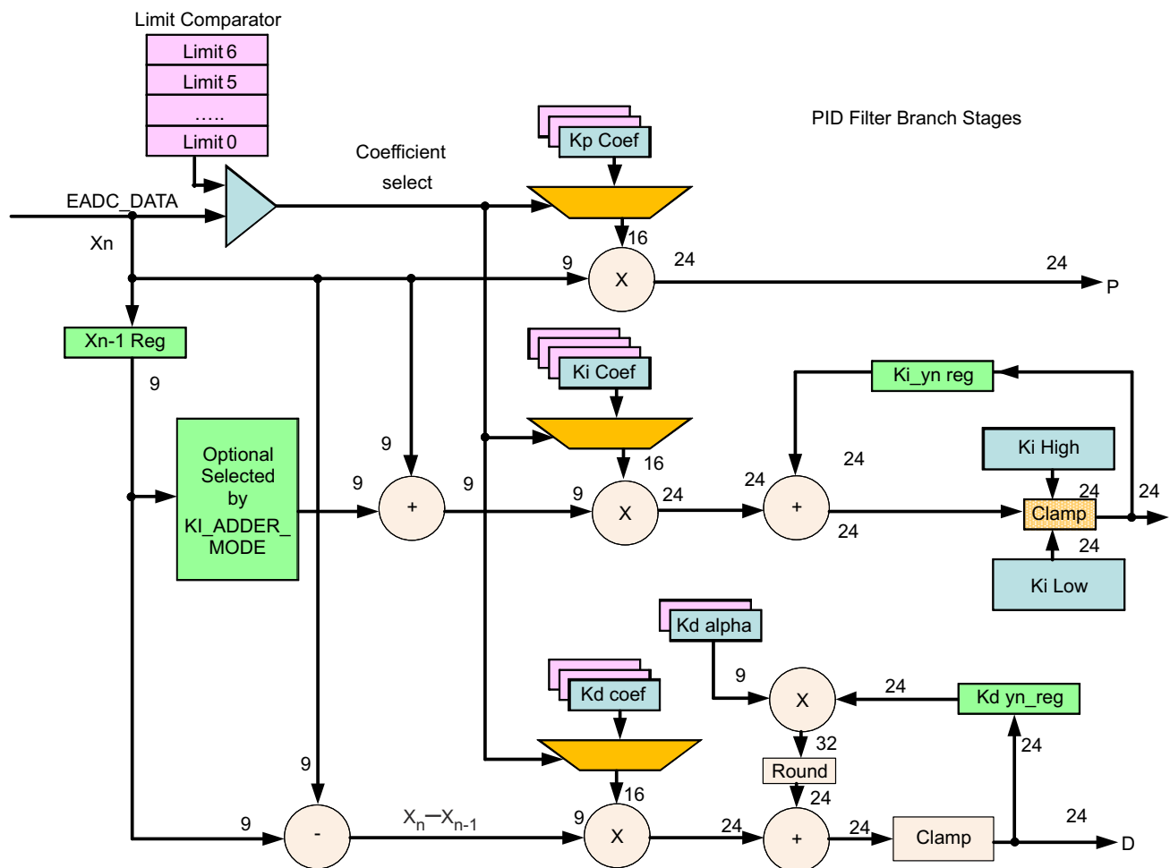
Figure 9-10. First Section of the Filter
