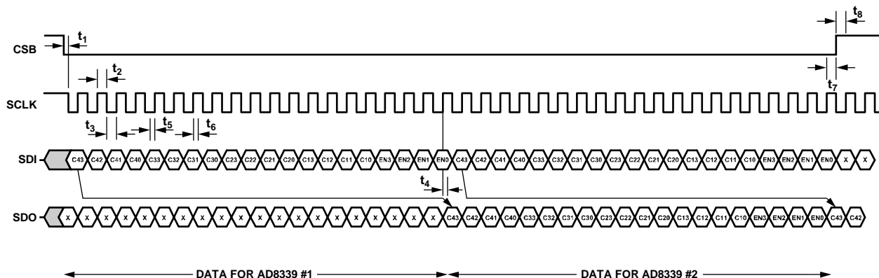
Figure 57. Timing Diagram
