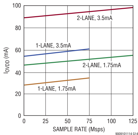
I_{VDD} vs Sample Rate, 5MHz Sine Wave Input, -1dBFS
