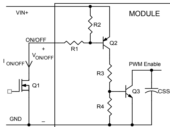
Figure 28. Circuit configuration for using positive logic On/Off.
