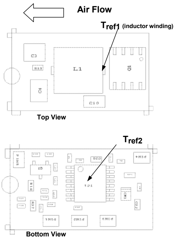
Figure 32. Tref Temperature measurement location.
