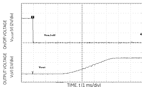
Figure 15. Typical Start-Up Using Remote On/Off with Low-ESR external capacitors (7x150µF Polymer)
