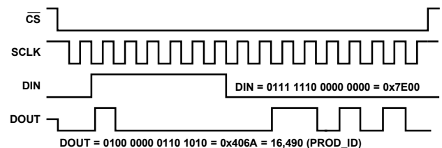
Figure 32. SPI Read Example, Second 16-Bit Sequence
