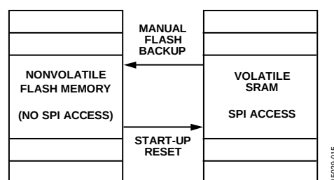
Figure 34. SRAM and Flash Memory Diagram
