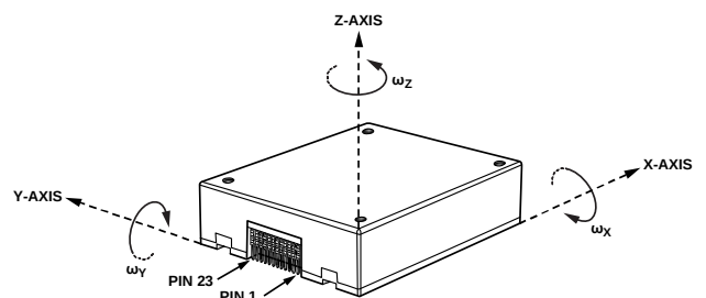
Figure 35. Gyroscope Axis and Polarity Assignments
