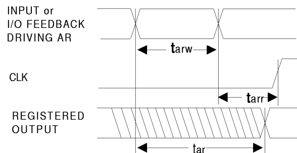
Asynchronous Reset
