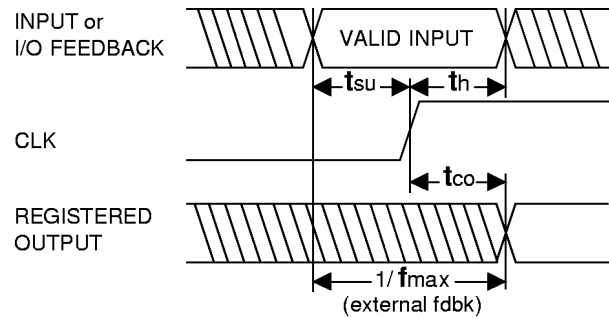
Registered Output
