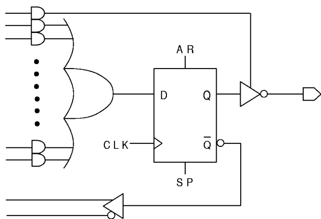
ACTIVE LOW
