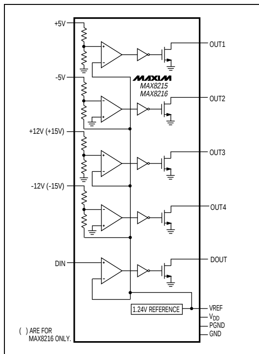
Figure 1. Block Diagram
