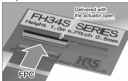
Ready to insert FPC/FFC
