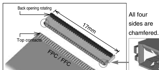
Easy FPC/FFC insertion
