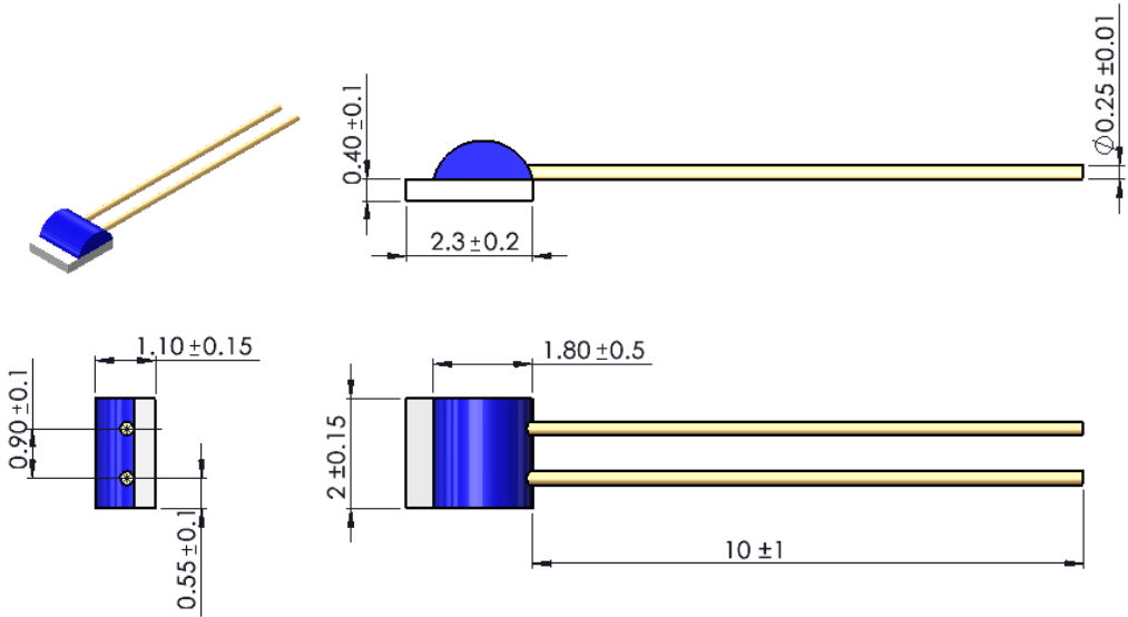
Figure 3: PTFC outline dimensions (mm)
