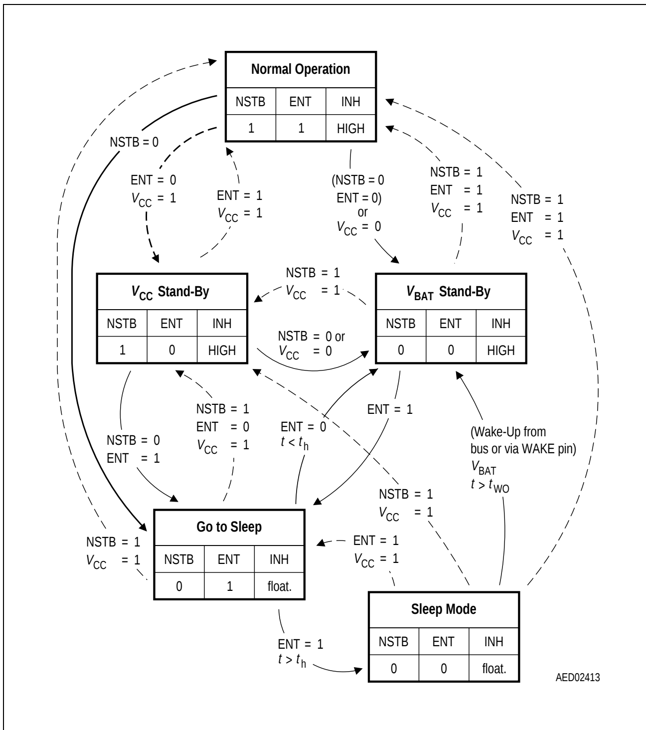
Figure 4 State Diagram
