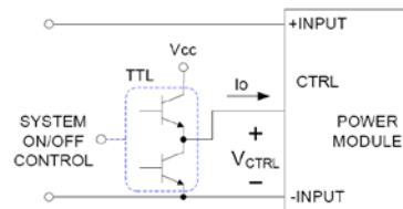
Level Control Using TTL Output
