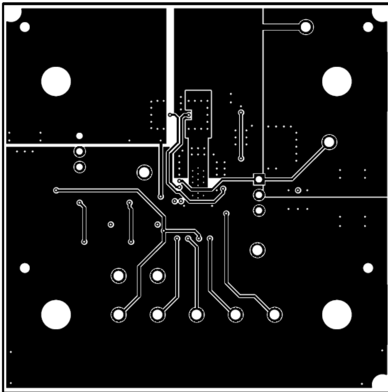
Figure 6. Layer 3 Routing
