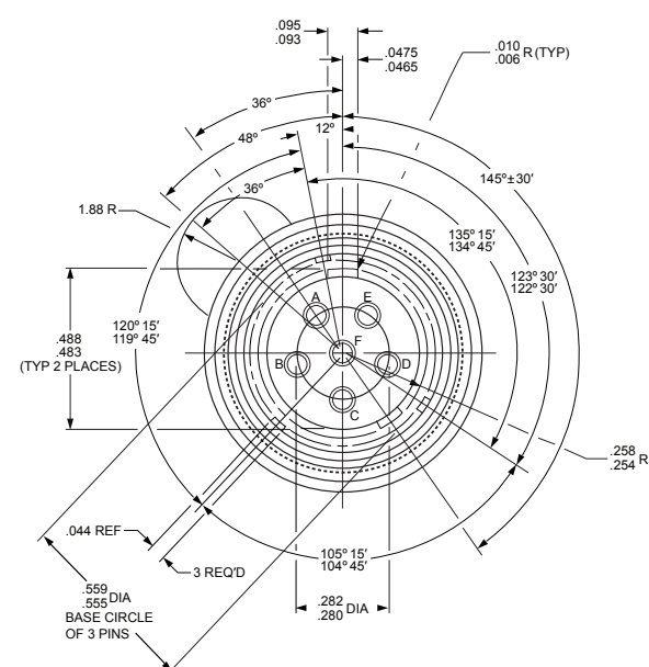
6-pin Insert Layout :
