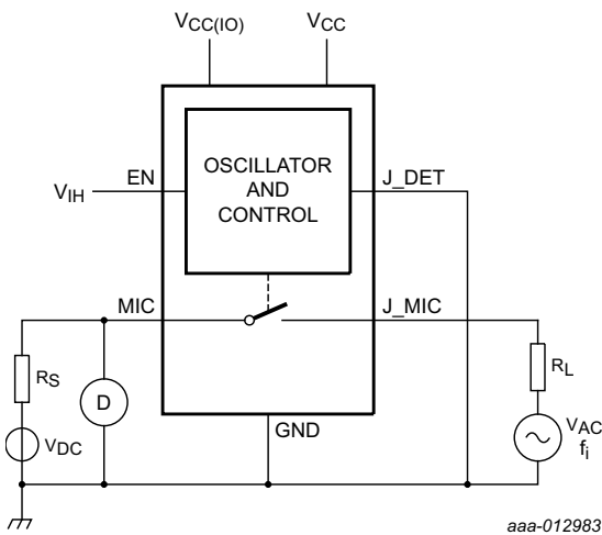
Fig 13. Test circuit for measuring total harmonic distortion
