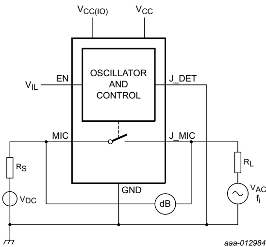
Fig 14. Test circuit for measuring isolation (OFF-state)
