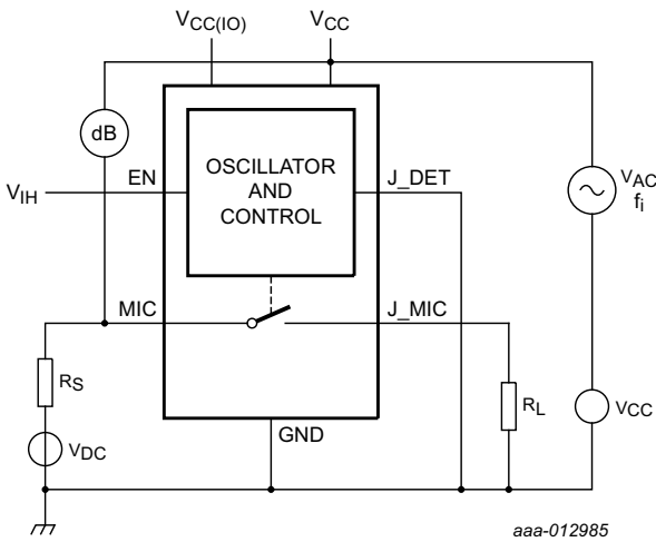
Fig 15. Test circuit for measuring the power supply rejection ratio
