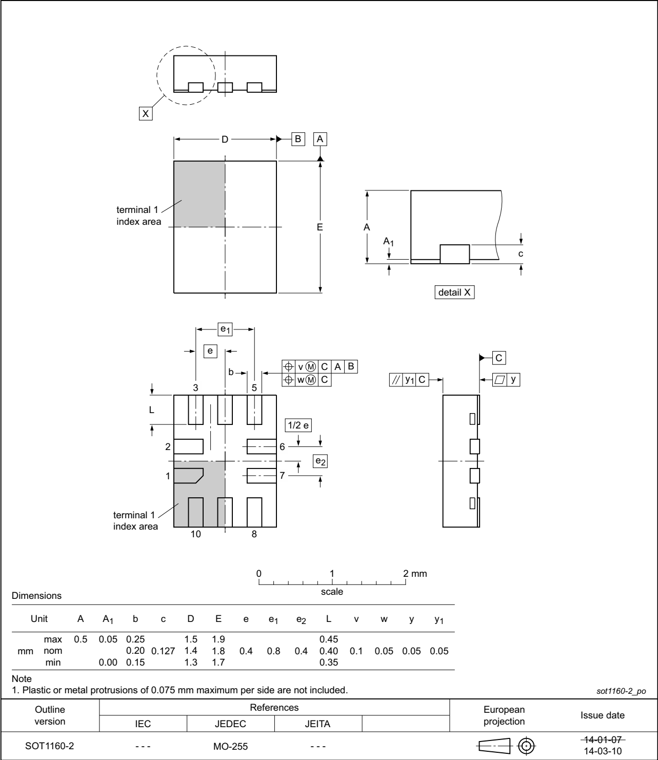
Fig 21. Package outline XQFN10 (SOT1160-2) package
