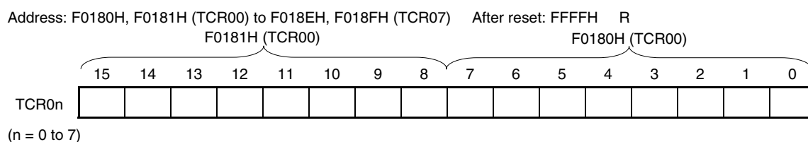
Figure 7-2. Format of Timer/Counter Register 0n (TCR0n)
