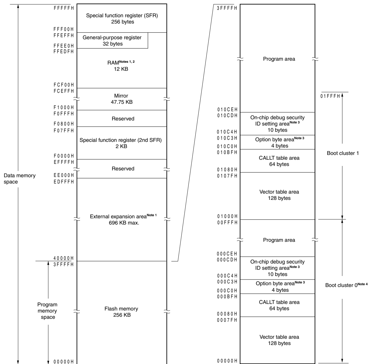
Figure 3-5. Memory Map (μPD78F1166, 78F1166A)
