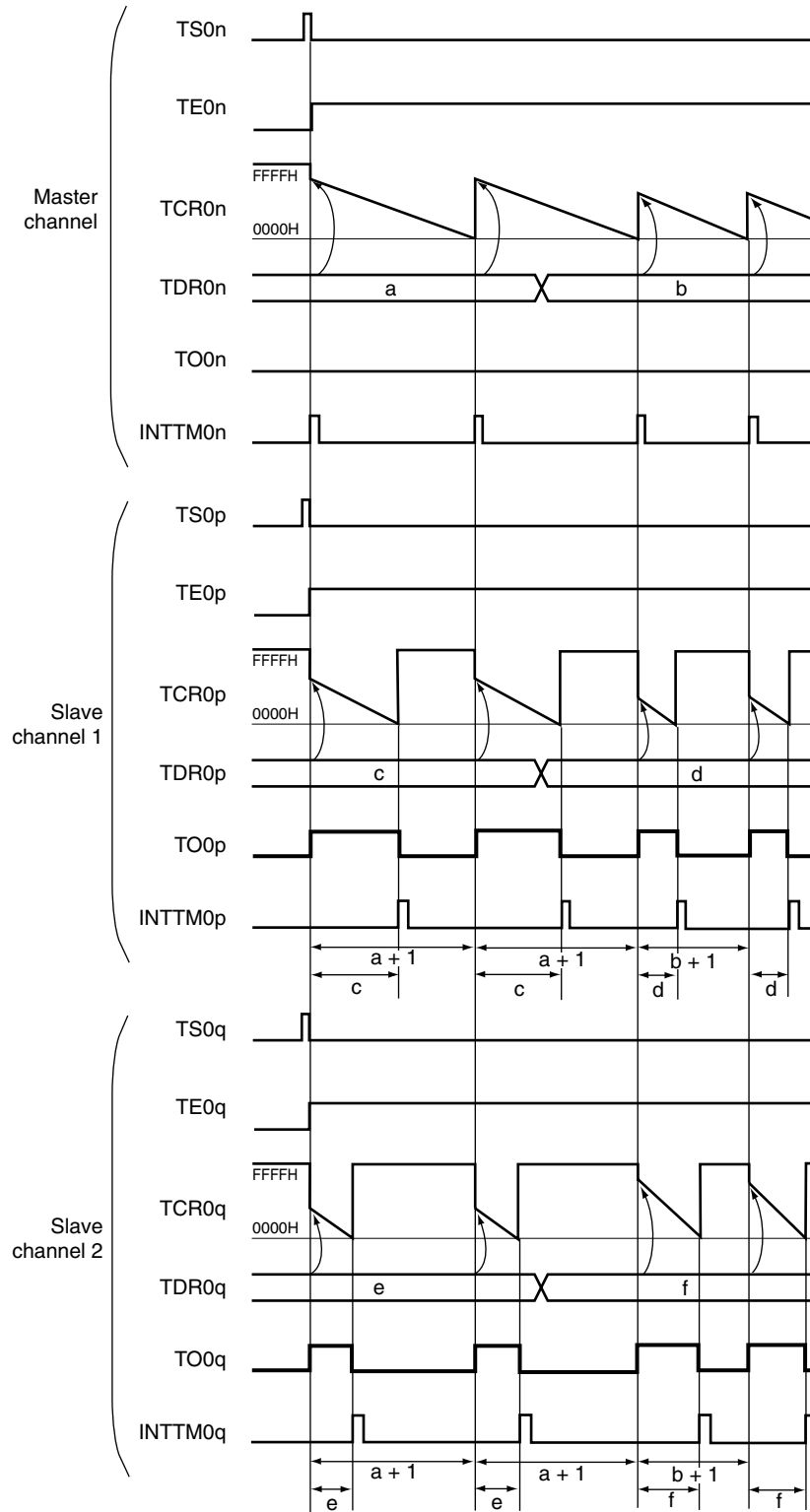
Figure 7-66. Example of Basic Timing of Operation as Multiple PWM Output Function (Output Two Types of PWMs)
