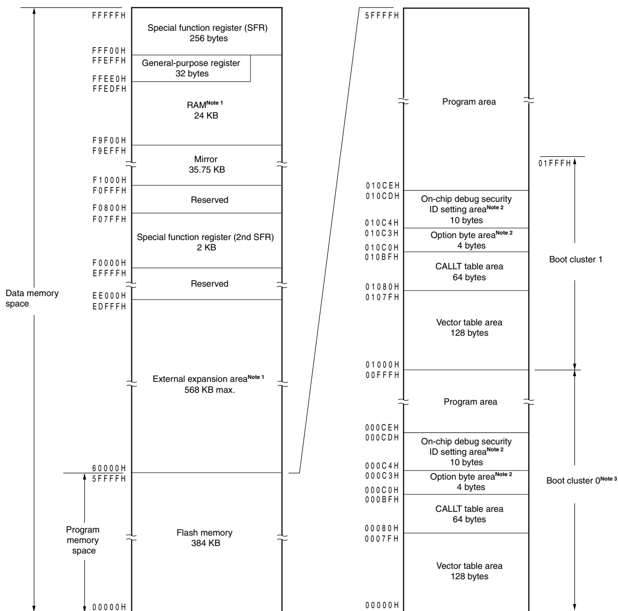
Figure 3-6. Memory Map (μPD78F1167, 78F1167A)
