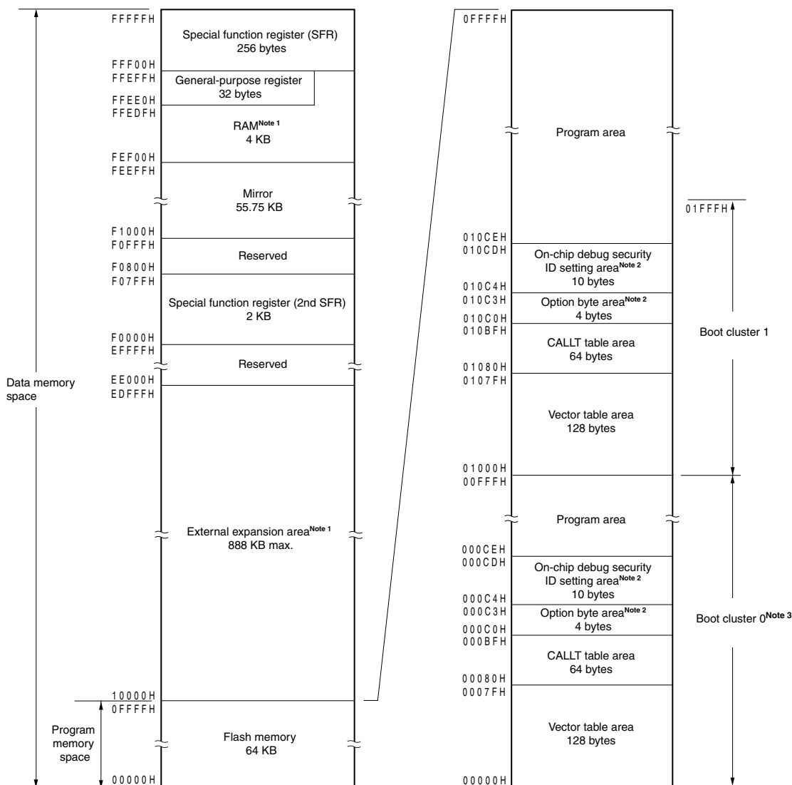
Figure 3-1. Memory Map (μPD78F1162, 78F1162A)
