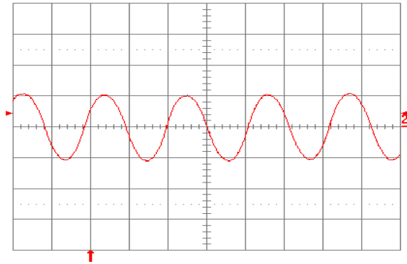
Fig. 2.5V.13: Input reflected-ripple current, i_e (100 mA/div.), measured at input terminals at full rated load current and V_{in} = 48 V. Refer to Fig. 2.5V.12 for test setup. Time scale: 1 \mu s/div.
