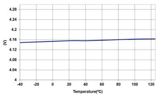
Vcc_UVLO_Start
