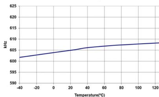
Frequency
