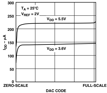
Figure 16. Supply Current vs. DAC Code
