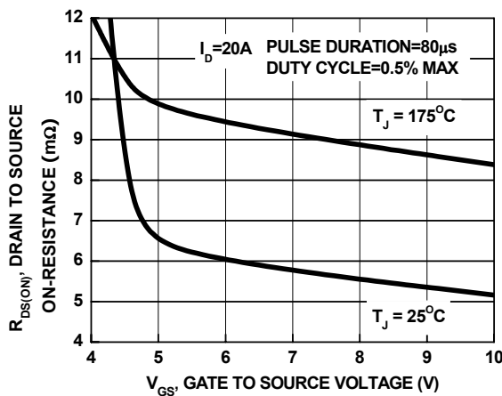
Figure 9. Drain to Source On-Resistance vs Gate to Source Voltage
