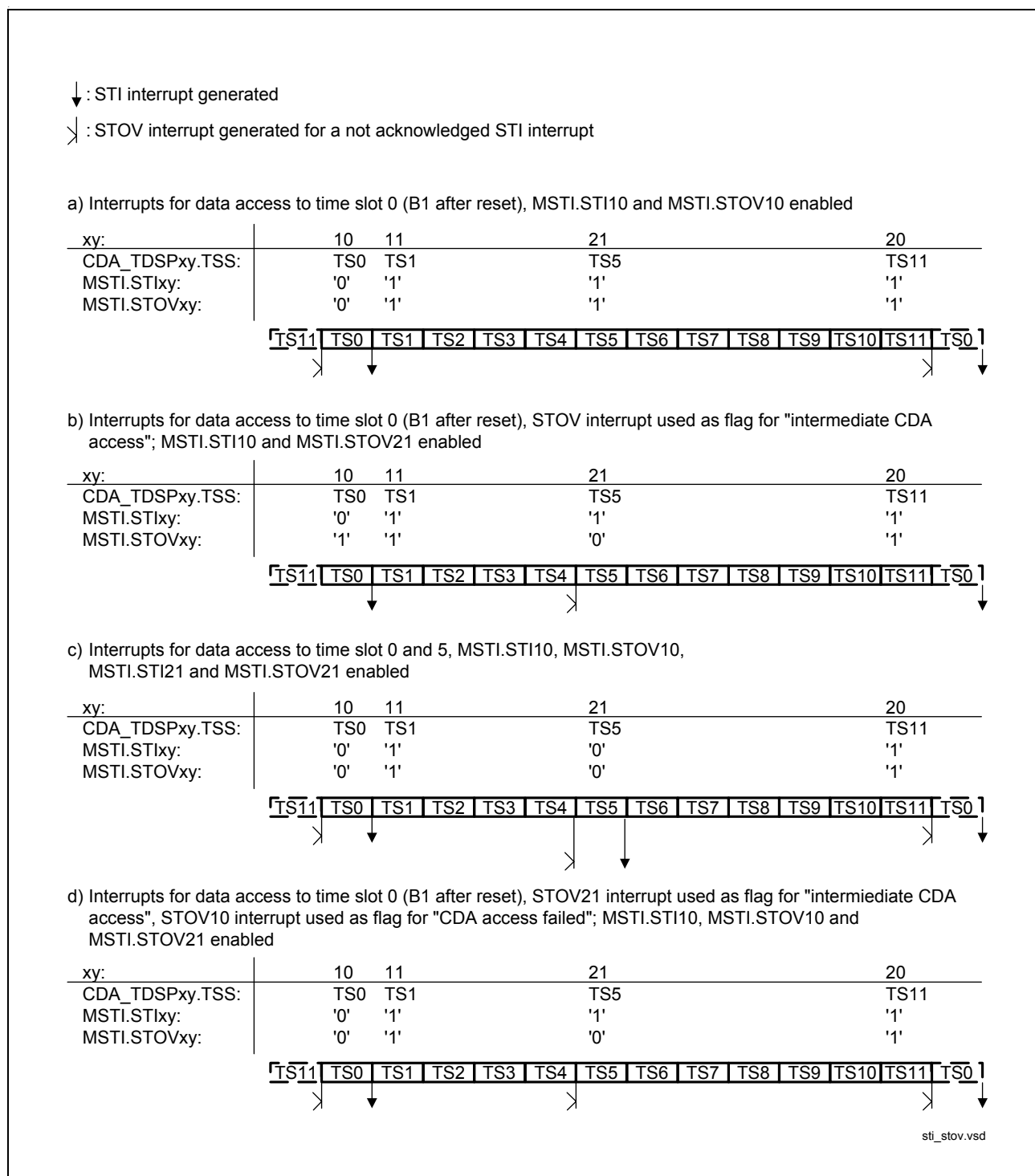
Figure 58 Examples for the Synchronous Transfer Interrupt Control With One Enabled STIxy
