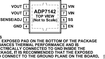
Figure 5. 8-Lead SOIC Pin Configuration
