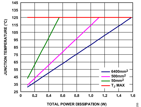
Figure 55. SOIC, T_A = 25^\circ\text{C}
