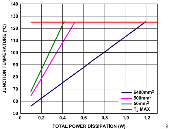
Figure 56. SOIC, T_A = 50^\circ\text{C}
