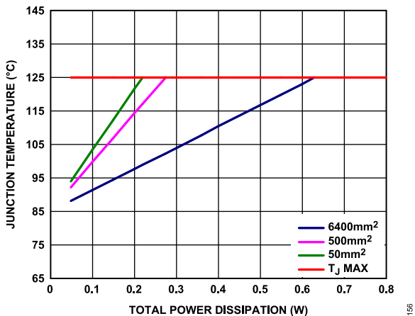
Figure 57. SOIC, T_A = 85^\circ\text{C}
