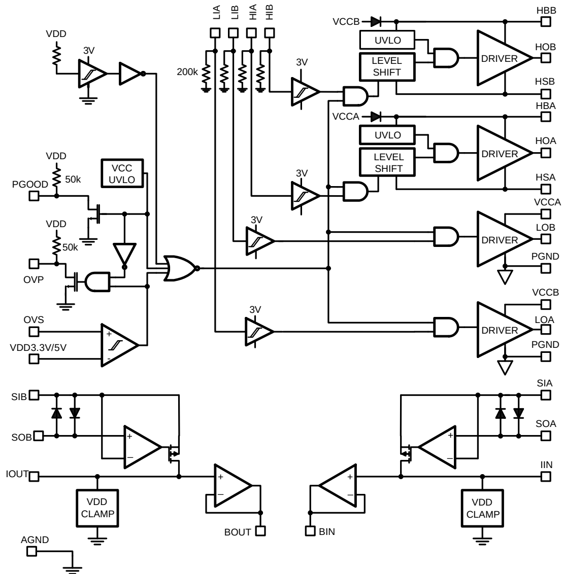
Figure 2. Block Diagram
