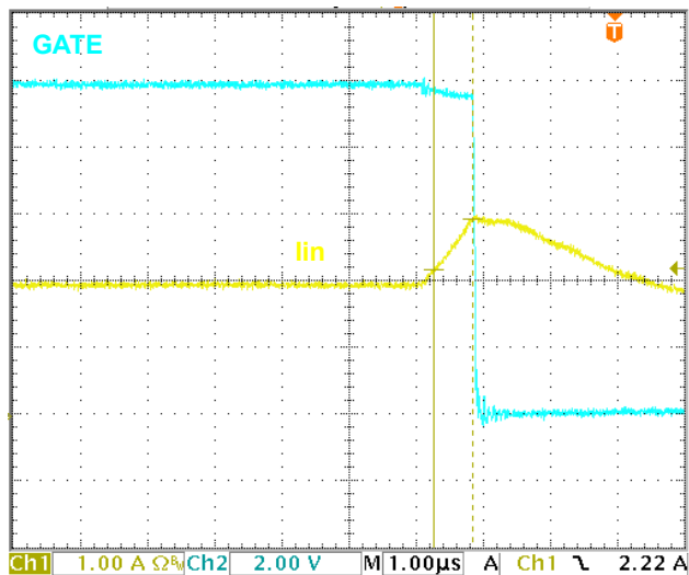
FIGURE 22. SHORTED OUTPUT GATE RESPONSE
