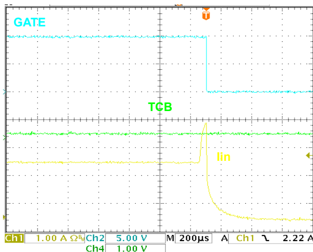
FIGURE 21. WOC CIRCUIT BREAKER OPERATION ZOOM
