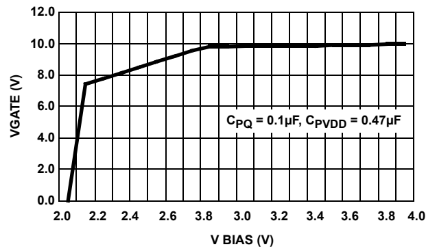
FIGURE 6. V_GATE vs V_BIAS
