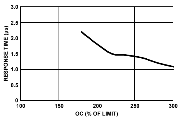
FIGURE 14. RESPONSE TIME vs I_O \cdot R_{SNS}
