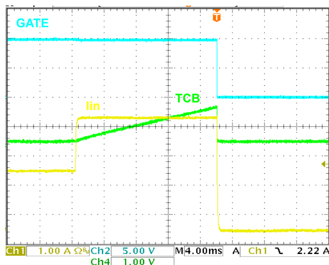
FIGURE 19. TRANSIENT TO 3.9A OC CIRCUIT BREAKER OPERATION
