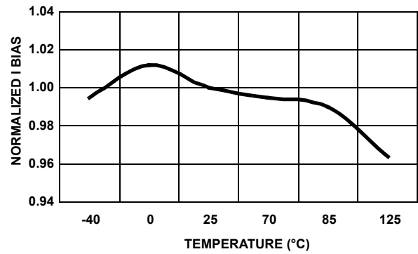
FIGURE 4. NORMALIZED I_BIAS (VBIAS = 3.3V) vs TEMPERATURE
