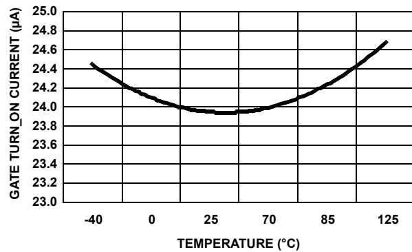
FIGURE 8. GATE TURN-ON CURRENT vs TEMPERATURE
