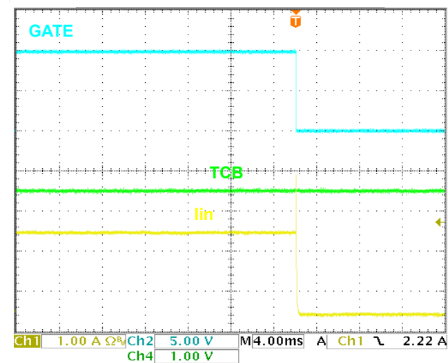
FIGURE 20. WOC CIRCUIT BREAKER OPERATION
