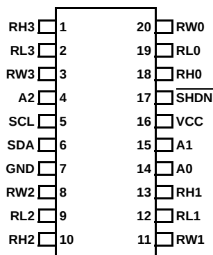
ISL22346 (20 LD TSSOP) TOP VIEW
