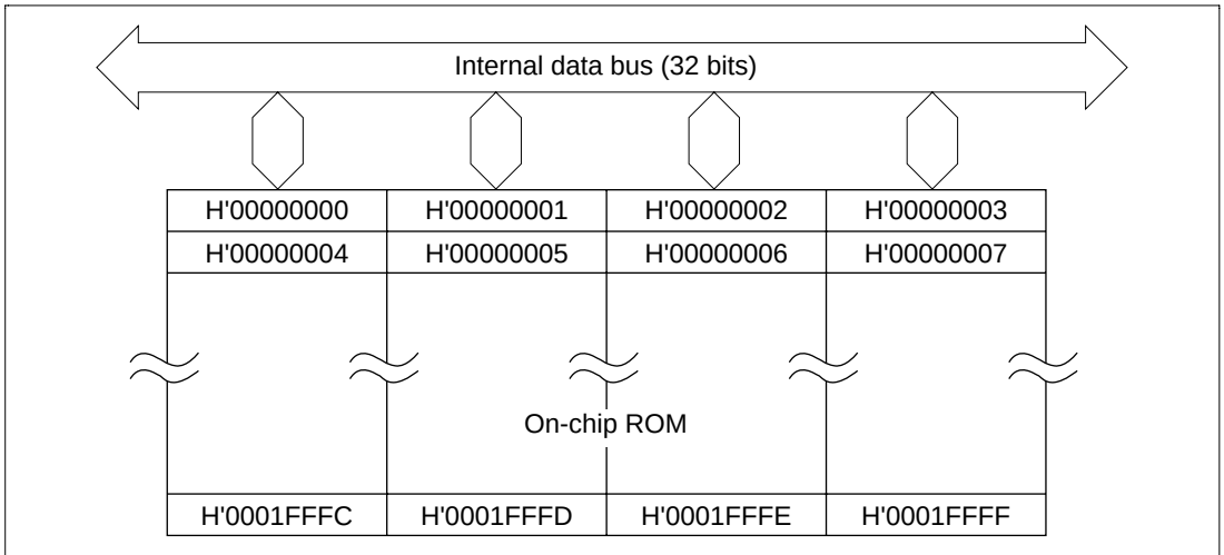
Figure 21.1 PROM Block Diagram
