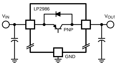
Figure 33. Inherent Diode
