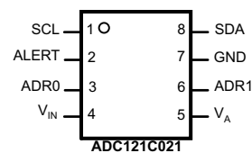
Figure 3. 8-Pin VSSOP See DGK Package
