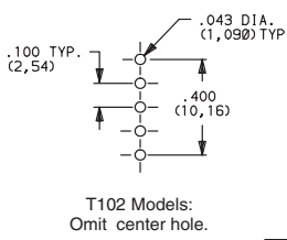
T101MH9V3BE SPDT
