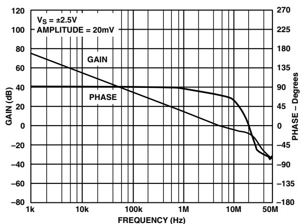
TPC 6. Gain and Phase vs. Frequency
