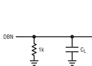
A. HI-Z TO V_{OH} AND V_{OL} TO V_{OH}
