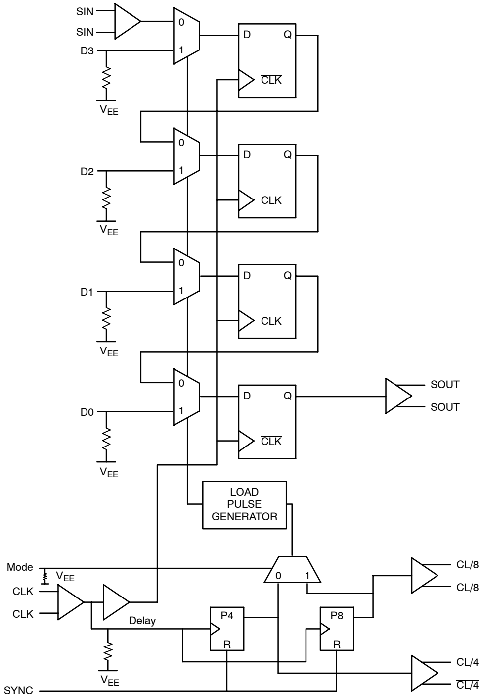
Figure 2. Logic Diagram
