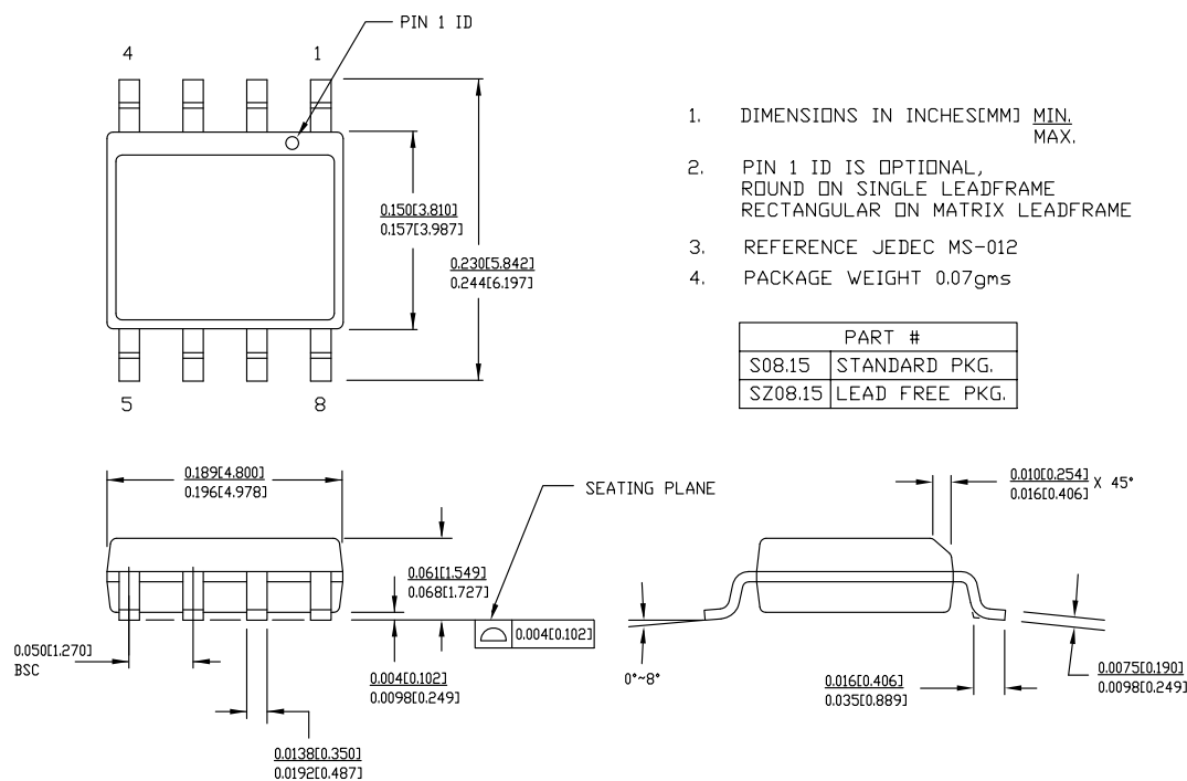
Figure 9. 8-Pin (150-Mil) SOIC S08 and SZ08
