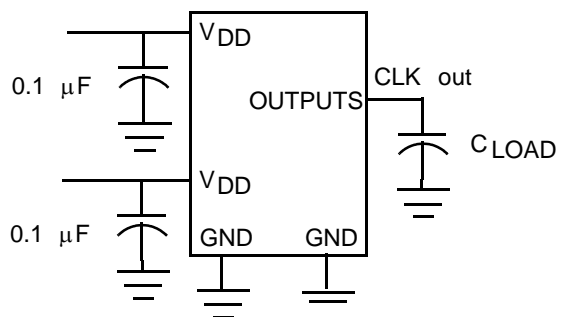
Test Circuit # 1
