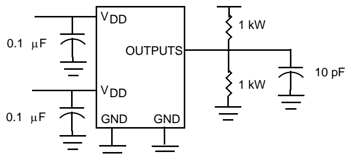
Test Circuit # 2
