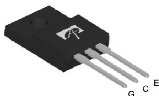
AOTF5B60D
