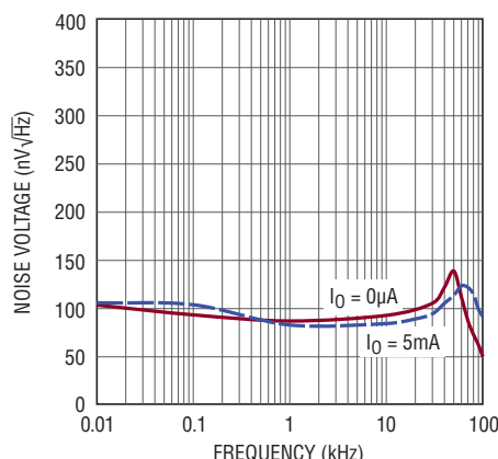
1.2V Output Voltage Noise Spectrum
