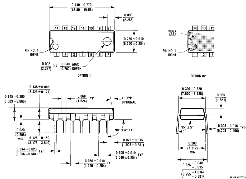
Molded Dual-In-Line Package (N) Order Number DM74ALS09N Package Number N14A
