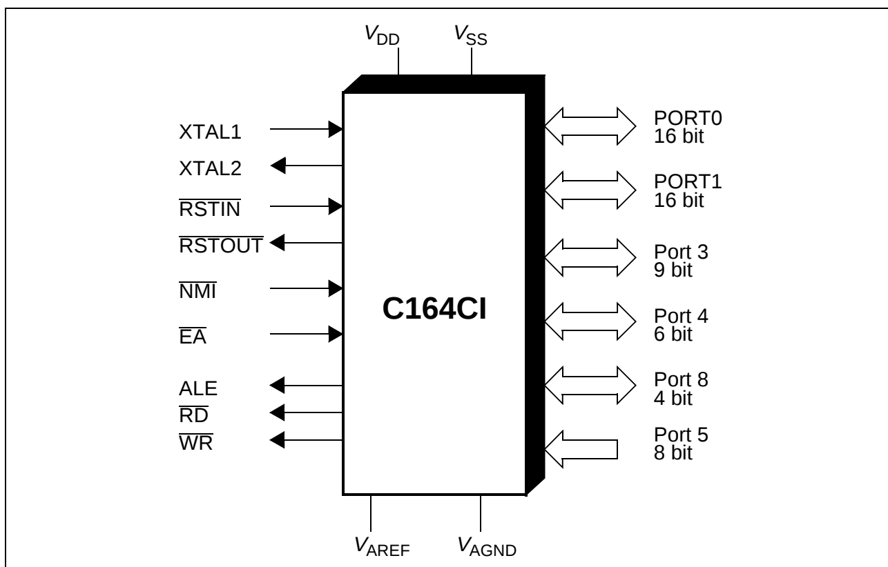
Figure 1 Logic Symbol
