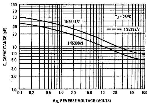
FIGURE 12 — JUNCTION CAPACITANCE
