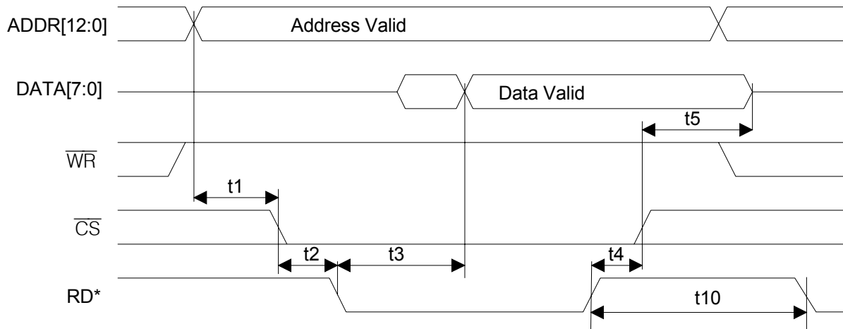
Figure 19-7 Intel Bus Read Timing (BTS = 0)
