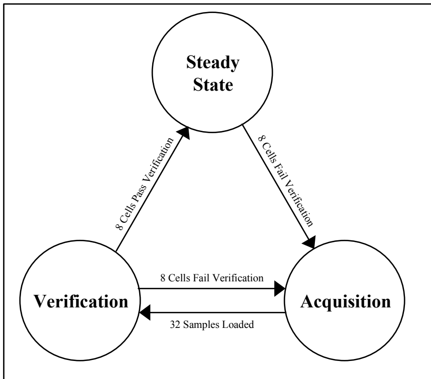
Figure 8-4 Receive DSS Scrambler Synchronization State Diagram
