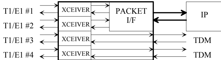
Figure 3-3 IP Over 2 Ports, TDM Over 2 Ports
