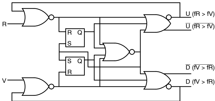
Figure 1. Logic Diagram
