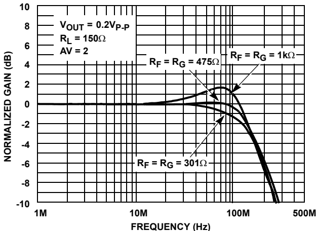
FIGURE 4. SMALL SIGNAL GAIN vs R_F , R_G
