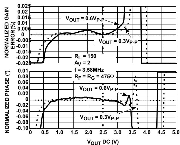
FIGURE 6. DIFFERENTIAL GAIN - PHASE
