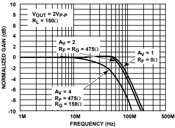
FIGURE 2. LARGE SIGNAL GAIN vs FREQUENCY for VARIOUS GAINS
