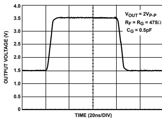
FIGURE 8. LARGE SIGNAL TRANSIENT RESPONSE; A_V = 2
