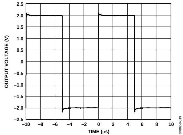
Figure 19. Large Signal Pulse Response Quad Op Amp Circuit (Figure 29) V_S = \pm 12\text{ V} , R_{LOAD} = 100\ \Omega , G = +5 , 4\text{ V Step}
