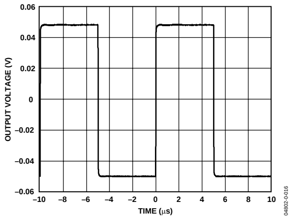
Figure 16. Small Signal Pulse Response Quad Op Amp Circuit (Figure 29) V_S = \pm 12\text{ V} , R_{LOAD} = 100\ \Omega , G = +5 , 100\text{ mV Step}
